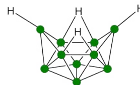
\text{B}_{10}\text{H}_{14}
