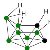
4,5-C 2 B 7 H 13
