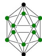
1,12\text{-C}_2^{10}\text{B}_{10}\text{H}_{12}
