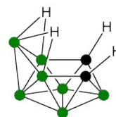
4,6\text{-C}_2\text{B}_7\text{H}_{13}
