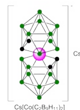
Cs[Co(C 2 B 9 H 11 ) 2 ]
