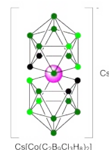
Cs[Co(C 2 B 9 Cl 3 H 8 ) 2 ]
