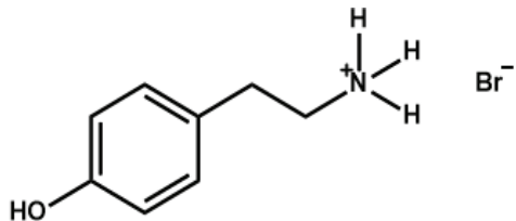
4-Hydroxyphenethylammonium bromide
