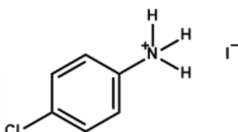
4-Chlorophenylammonium iodide
