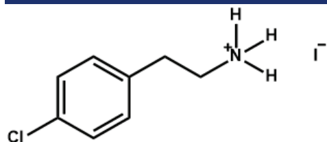
4-Chlorophenethylammonium iodide
