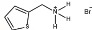
2-Thiophenemethylammonium bromide
