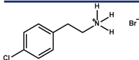
4-Chlorophenethylammonium bromide
