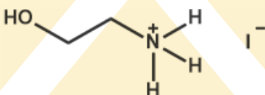
Ethanolammonium iodide
