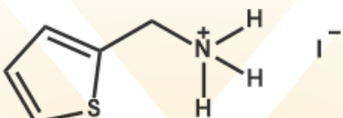
2-Thiophenemethylammonium iodide
