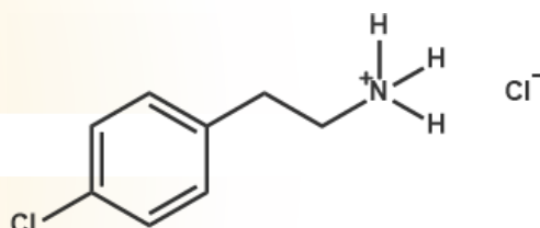
4-Chlorophenethylammonium chloride
