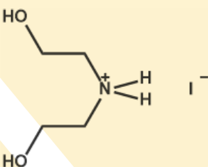
Diethanolammonium iodide
