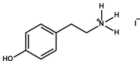
4-Hydroxyphenethylammonium iodide
