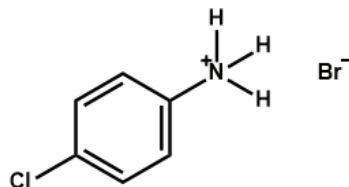
4-Chlorophenylammonium bromide
